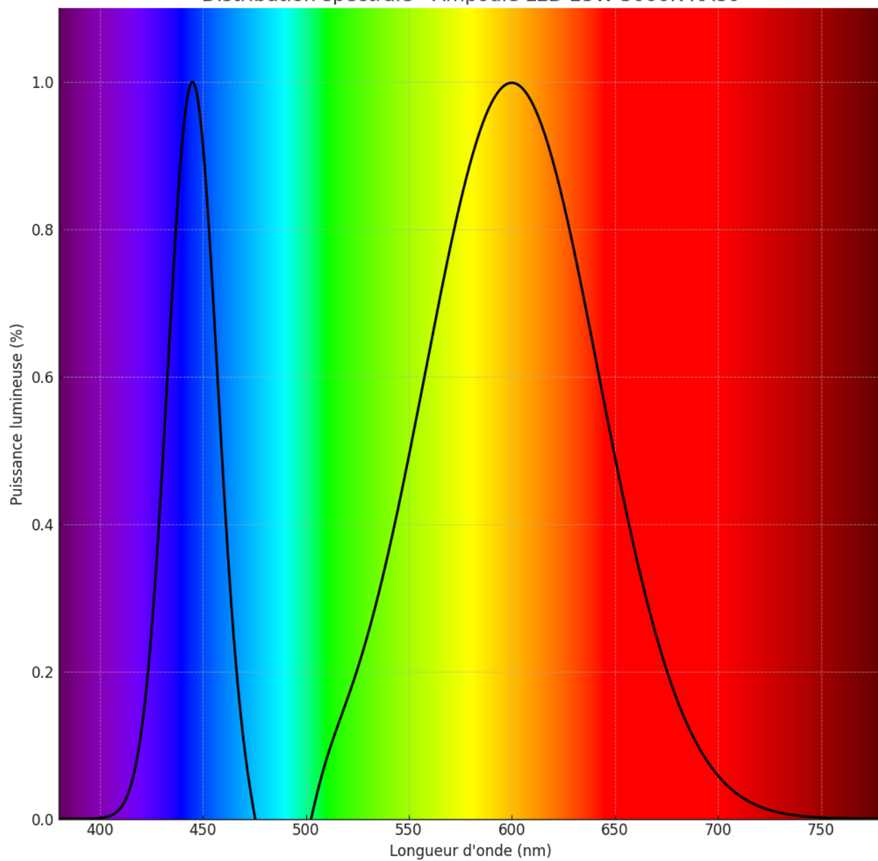
Distribution spectrale - Ampoule LED 25W 3000K RA80
