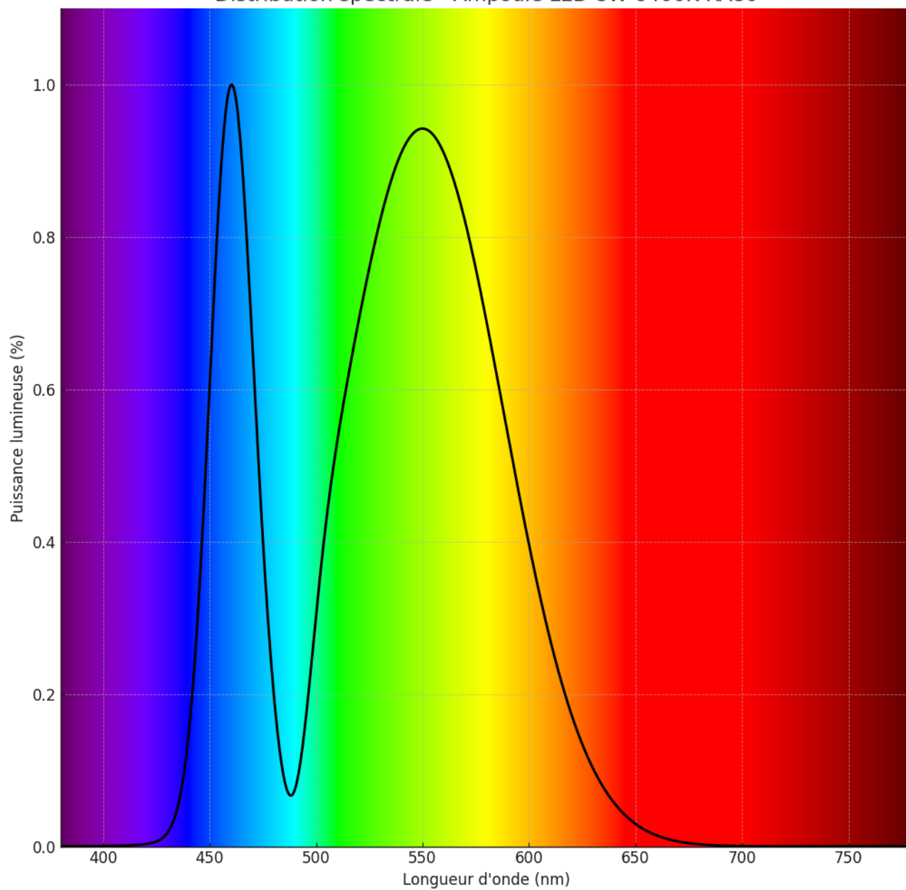
Distribution spectrale - Ampoule LED 8W 6400K RA80
