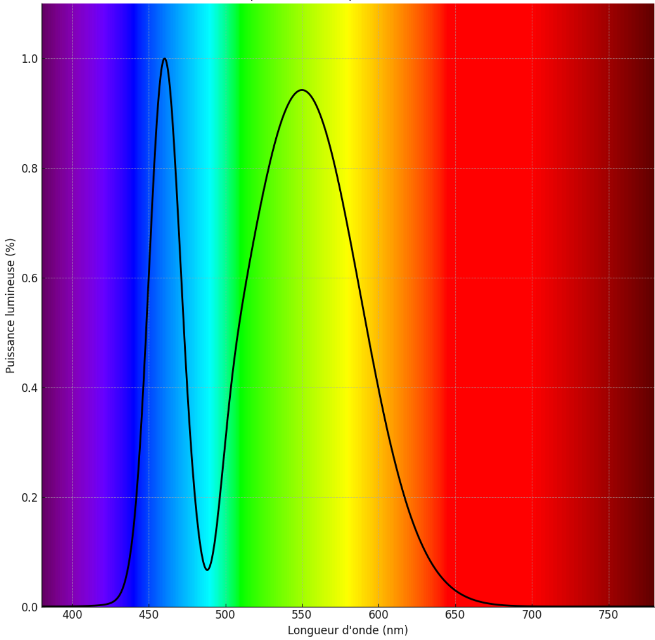
Distribution spectrale - Ampoule LED 8W 6400K RA80
