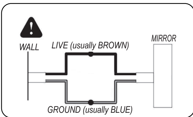
5.Connect the mirror with the main supply.
