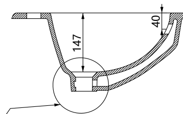
SECTION_VIEW A-A
