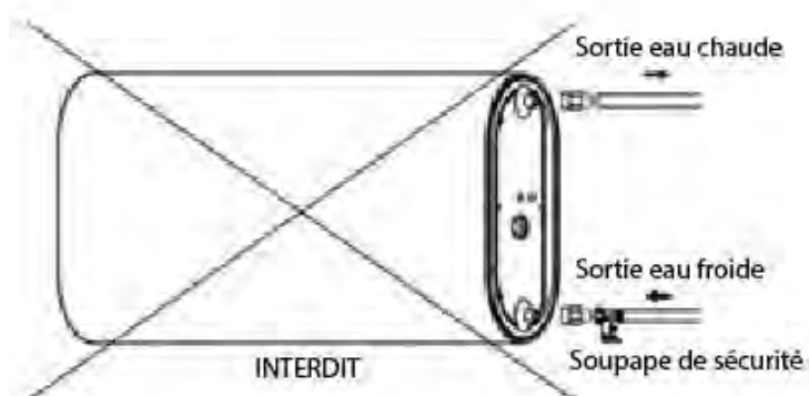
Figure 3 : Installation non-conforme
