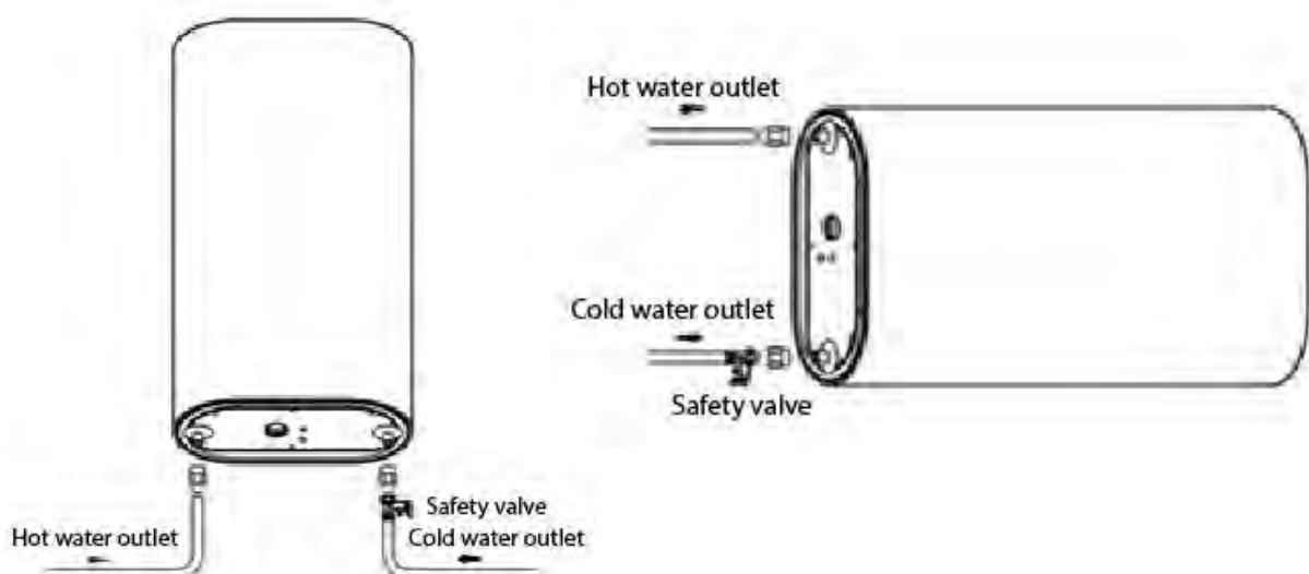
Figure 2: Compliant installation
