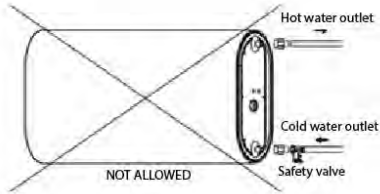
Figure 3: Non-compliant installation
