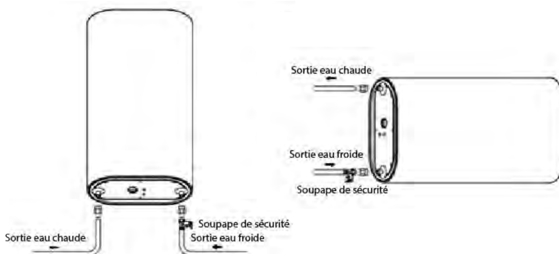
Figure 2 : Installation conforme
