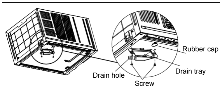
Bottom drainage
