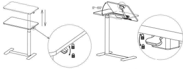
Height-lifting function
