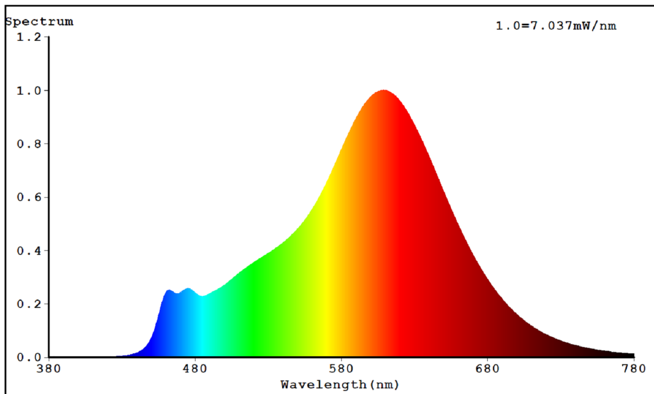
Spectral Distribution
