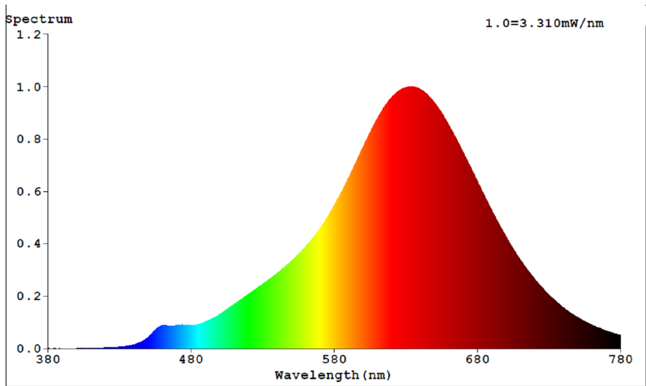
Spectral Distribution
