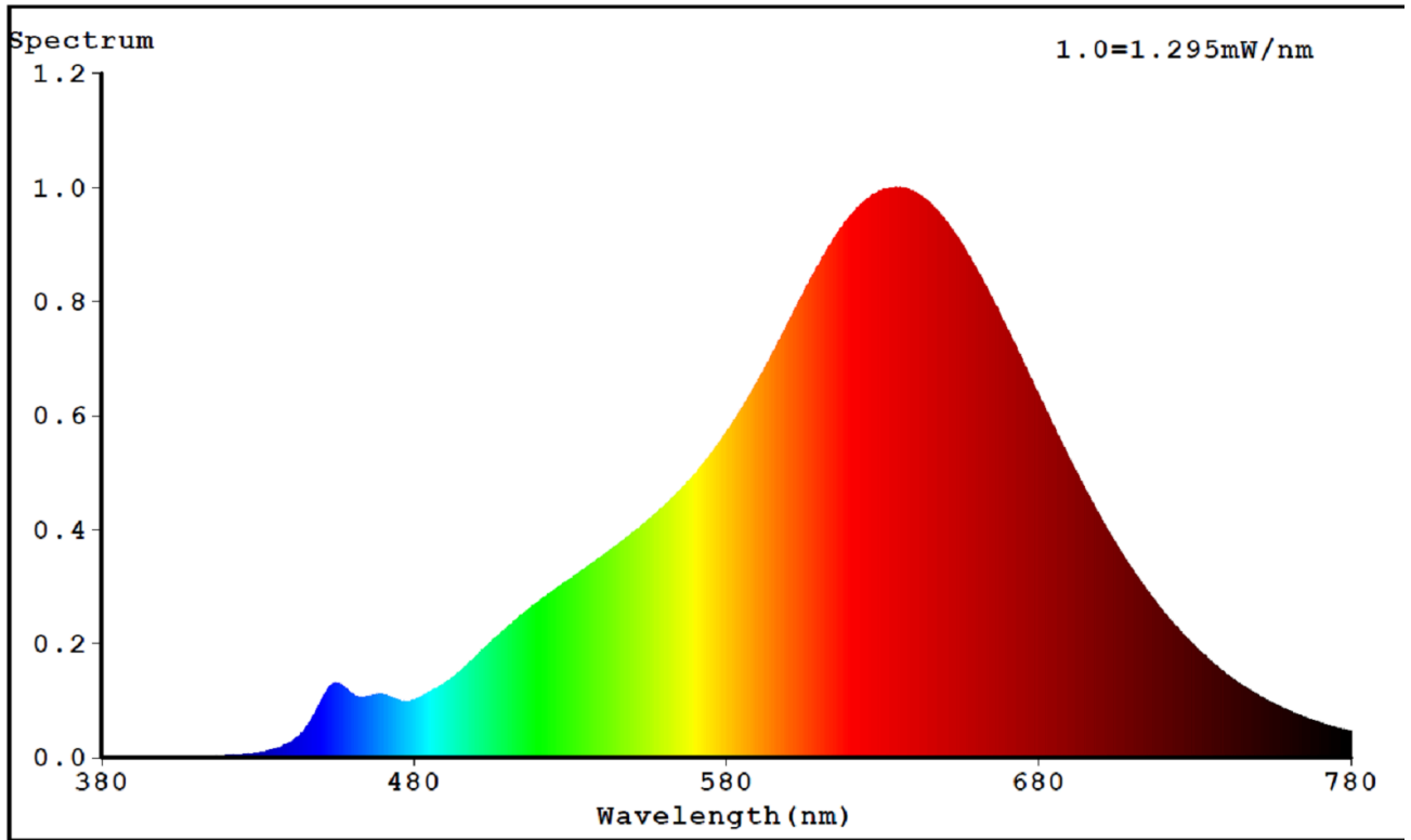
Spectral Distribution
