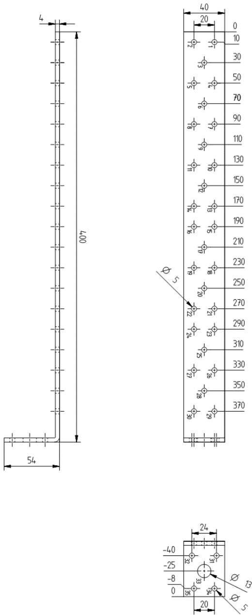
Figure A.80 hold-down 8799 4004 1D
