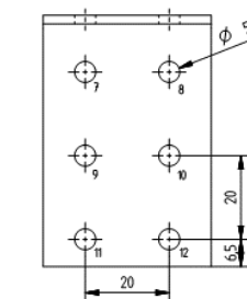
Figure A.10 Angle Bracket 8593 6060 1
