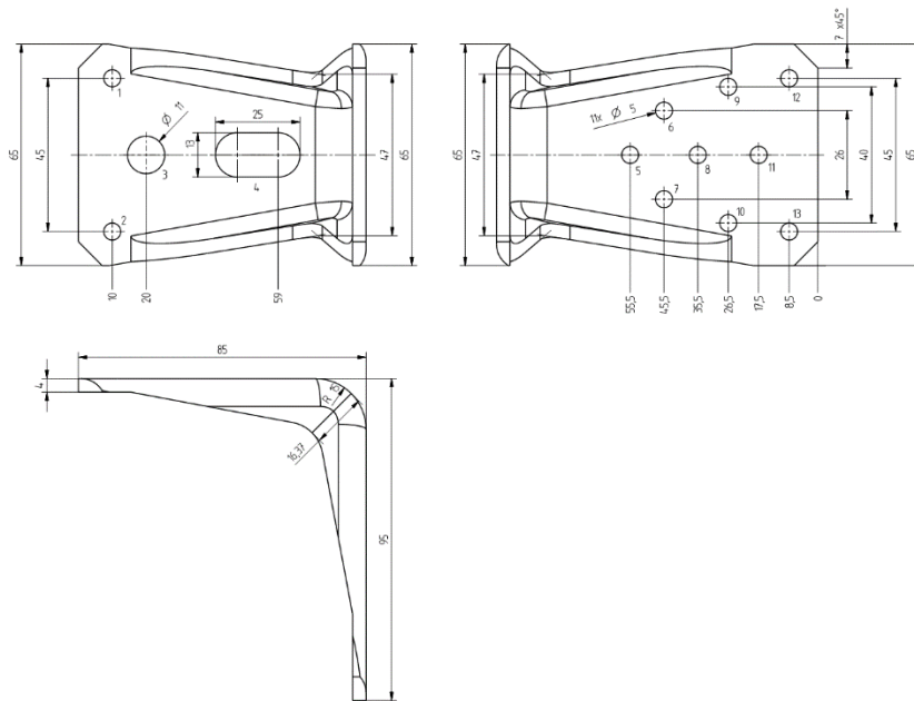
Figure A.1 Angle Bracket 8573 0095 1
