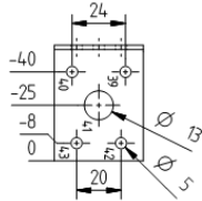
Figure A.71 hold-down 8795 5002 1D
