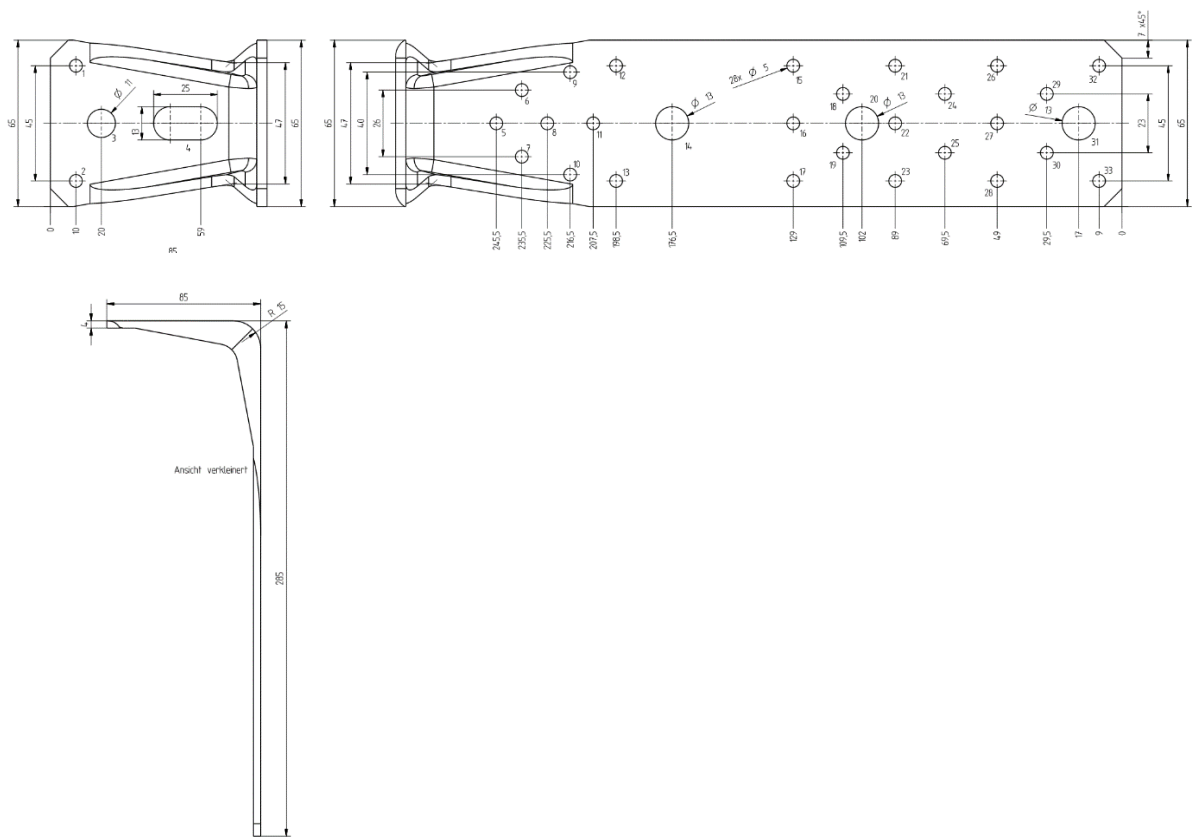
Figure A.3 Angle Bracket 8573 0285 1
