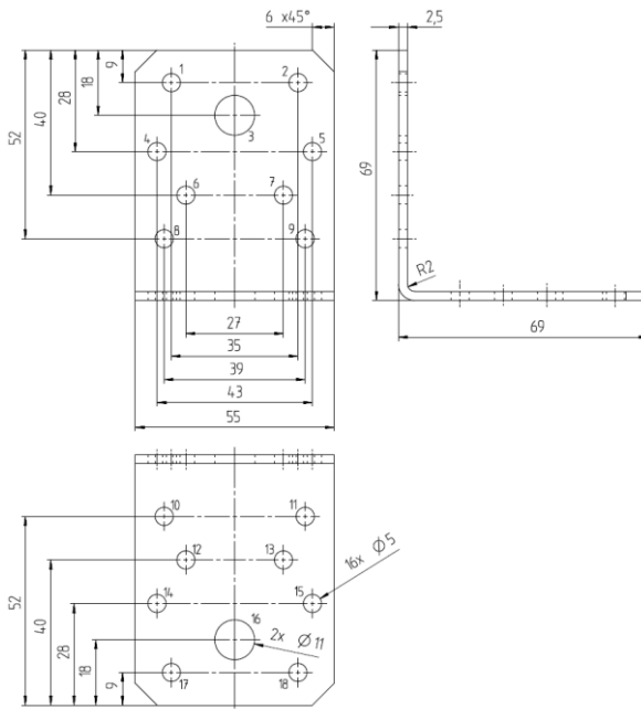
Figure A.24 Angle Bracket 8623
